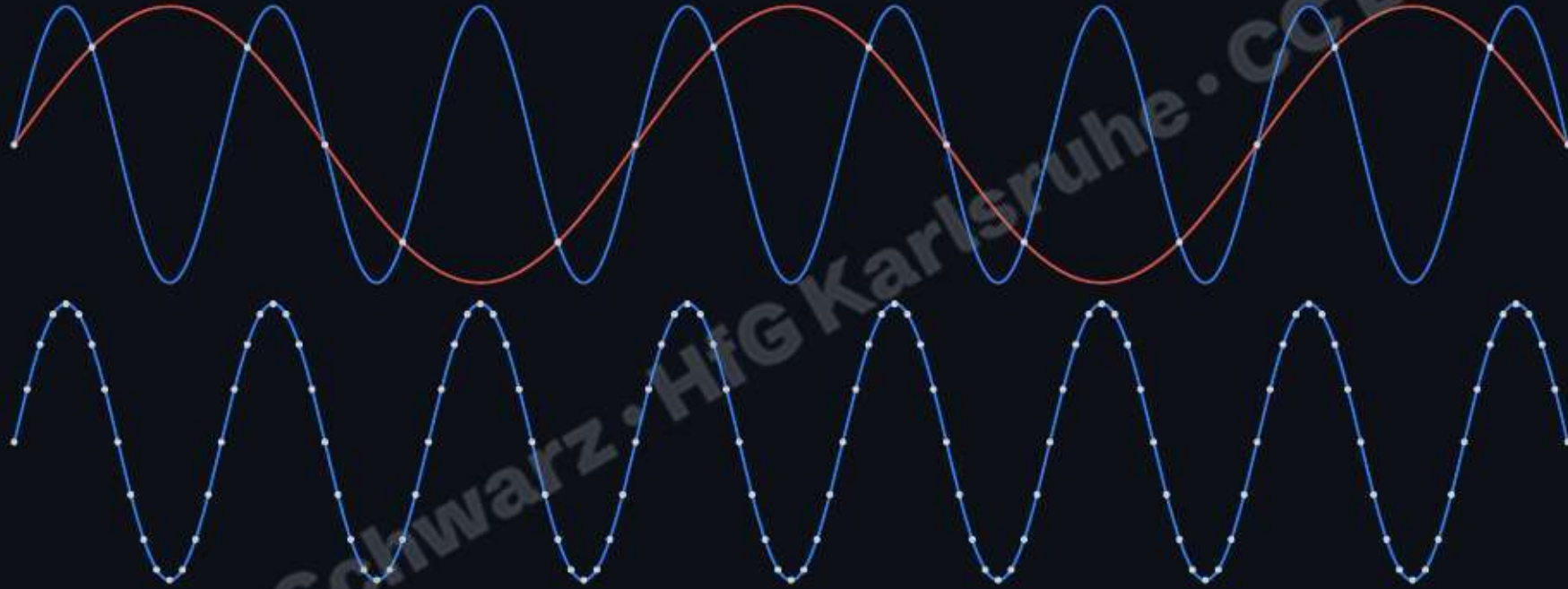
Undersampling (top) vs. correct sampling (bottom) of a sine wave
