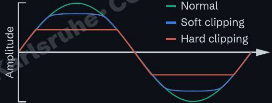
Hard clipping vs. soft clipping
